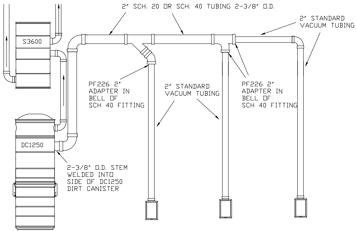
TYPICAL INSTALLATION OF THE S3600 WITH DC1250 (THIS IS A TWO USER SYSTEM)
